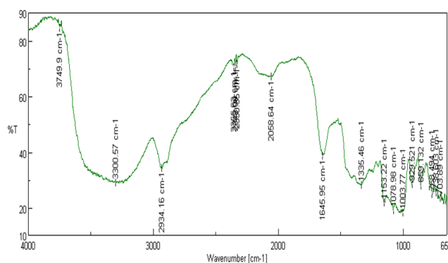
Figure 3: FTIR spectrum of elephant foot yam starch.
