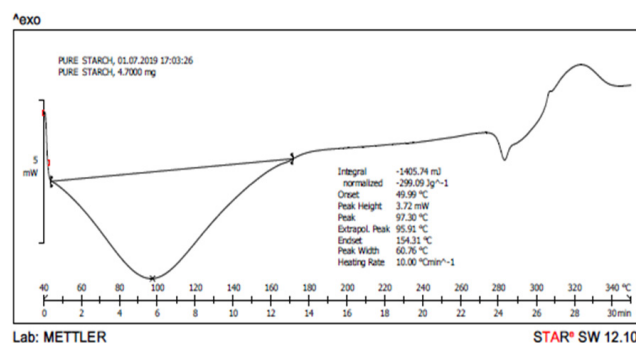
Figure 4: DSC thermogram of elephant foot yam starch.
