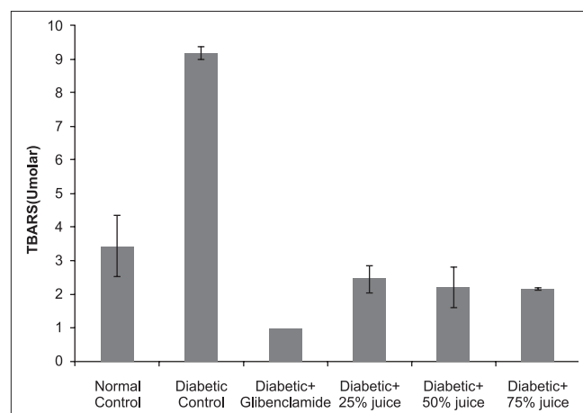
Figure 1: Effect of A. gangetica juice on TBARS level in plasma of the experimental rats (bars represent mean \pm SEM)
